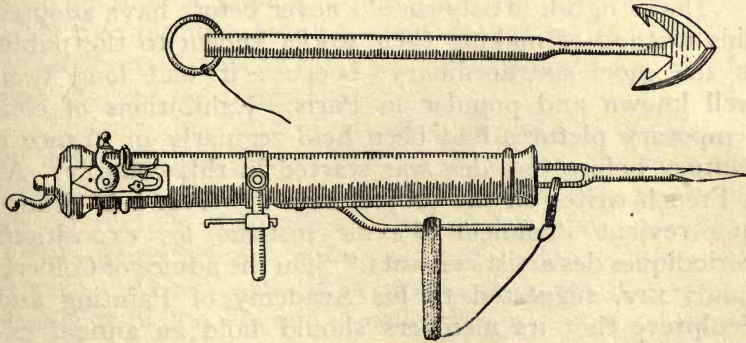
Abraham Stagholt's Gun-Harpoon (see p. 249).
